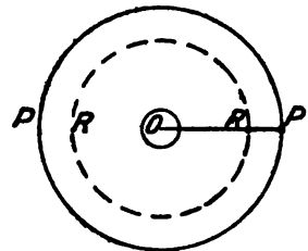
FIG. 32.—ANGULAR VELOCITY
